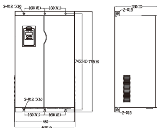
图E(S5100-4T75G~4T110G)
