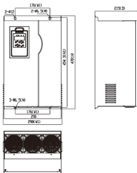
图C(S5100-4T30G)
