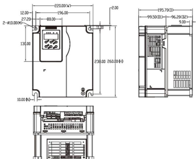
图A(S5100-4T5.5G~4T11G)
